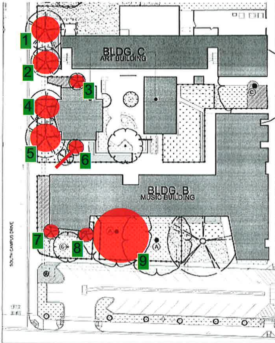
LANDSCAPE DEMOLITION & TREE PROTECTION PLAN
